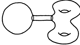
Figure 1: (\bar{M}, g_\varepsilon)
