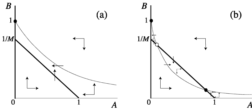
Fig. A.1 Phase plane for (A, B) projected on a plane Z = \text{constant} . Thick lines indicate the nullclines for A , and the dotted curve the nullcline for B . The shape of the dotted curve depends on the value of Z . Black point indicates the locally stable equilibrium point, and white point the unstable equilibrium point. (a) The equilibrium point is only (A, B) = (0, 1) . (b) Three equilibrium points appear.
